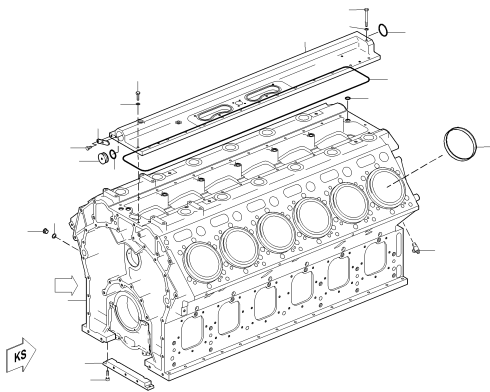
CRANKCASE UPC.06A01 2072
