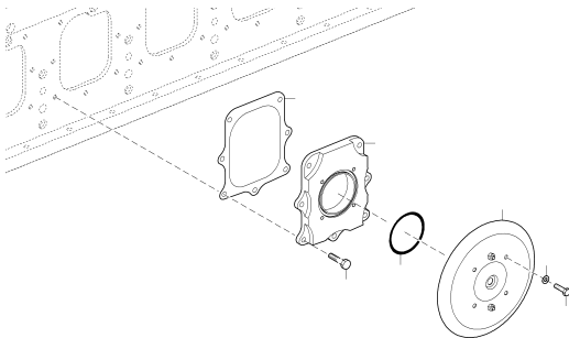
CVR CYL BLK ACCESS W/SAFETY VLV MARINE 0 UPC.06A01F0001
